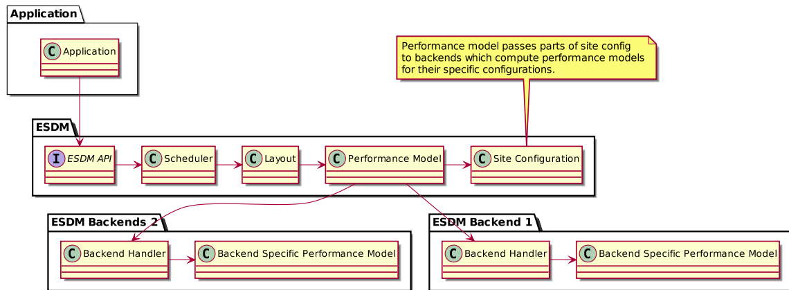
Figure 6.4.: An application that is using ESDM interfaces through the ESDM API (which in many cases maybe only read/write calls). Eventually the scheduling component has consult the layout component wich is responsible for returning a list of Fragments which have to be read or written. To provide this list the performance model is used which in turn queries the available backends and the site configuration for an estimate.
