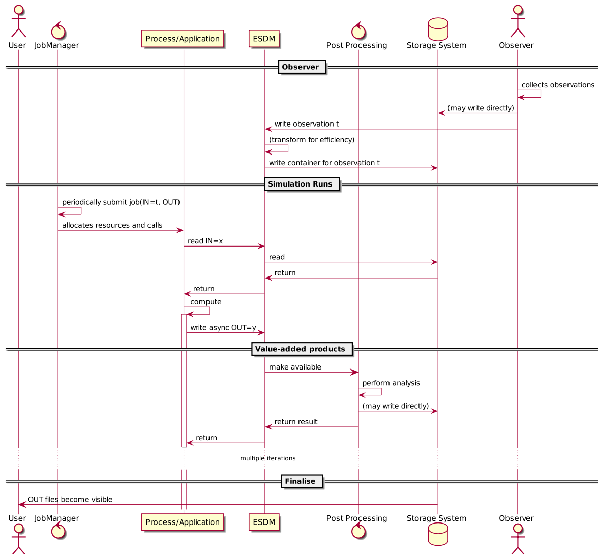
Figure 4.14.: Sequence Diagram
