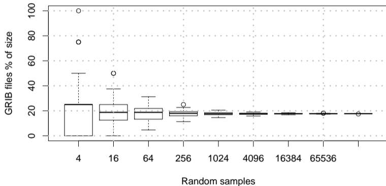
Figure: Simulation of sampling to compute proportions of types by size
