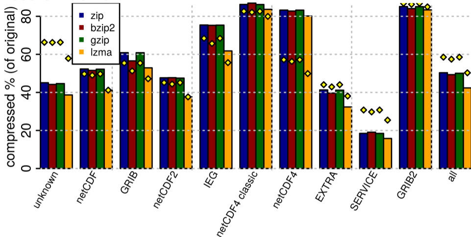
Figure: Arithmetic mean compression of the full data set for each scientific file format computed on file number. The column “all” shows the mean values for the whole data set. Yellow diamonds show compress % computed by file size
