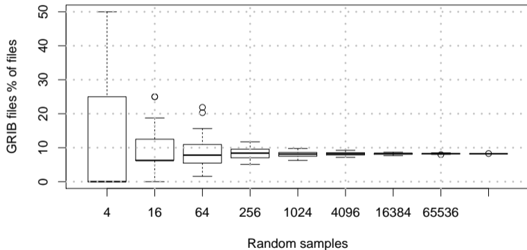
Figure: Simulation of sampling by file count to compute compr.% by file count
